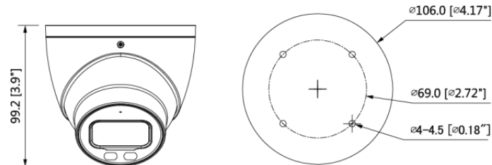
Figure 2-2 Model B (mm [inch])
