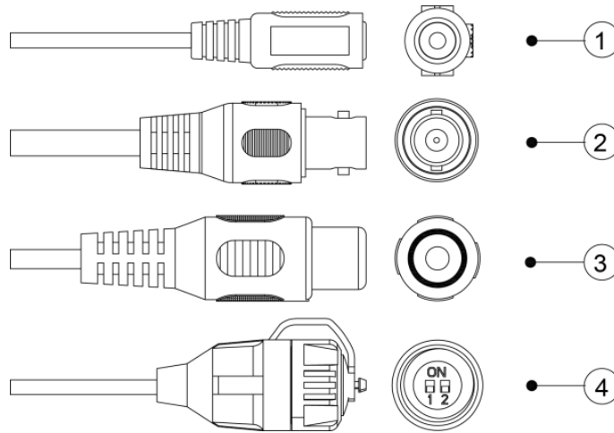
Figure 2-5 Cable port list
