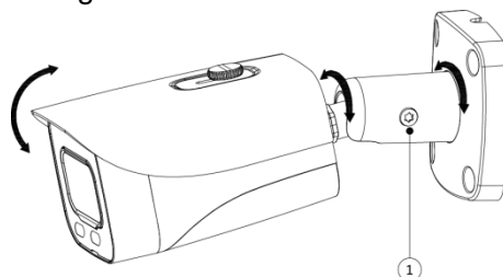
Figure 3-6 Model C installation
