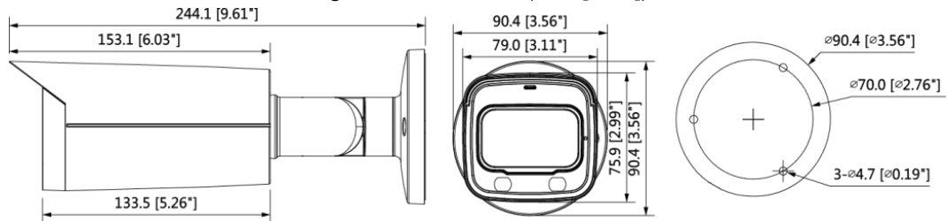
Figure 2-3 Model C (mm [inch])
