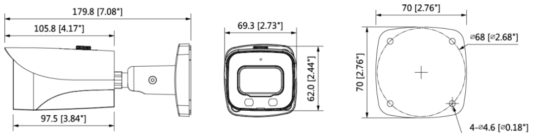
Figure 2-3 Model C (mm [inch])
